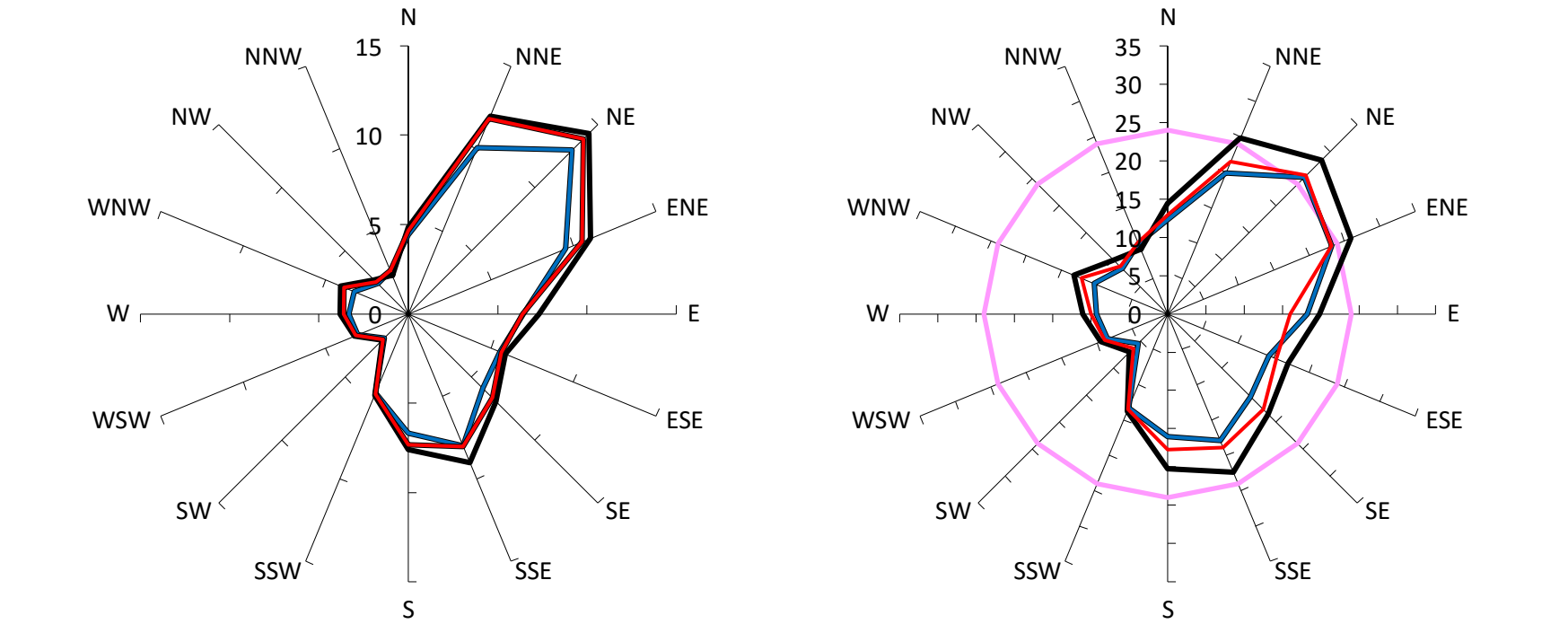
Comfort Criteria: 8m/s with 5% probability of exceedence
